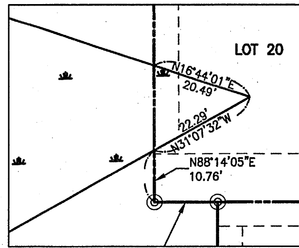
WETLAND DETAIL "A"
